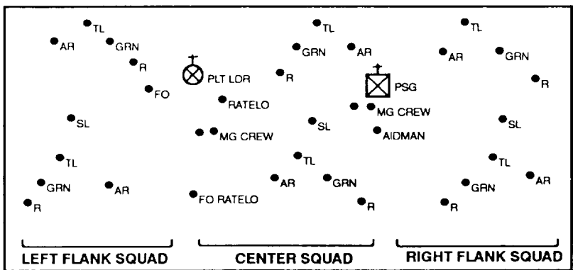
Figure 2-13. Platoon-line, squads-in-column.
